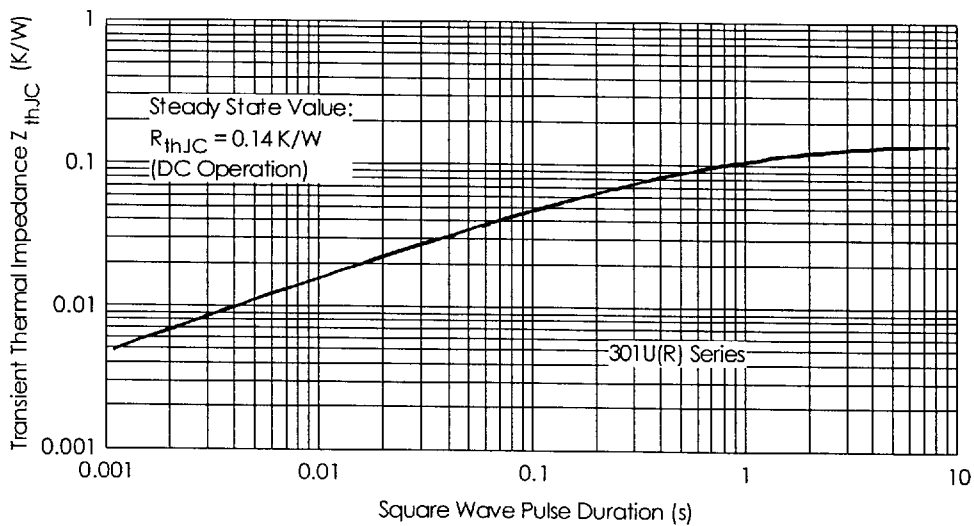
Fig. 15 - Thermal Impedance Z_{thJC} Characteristic
