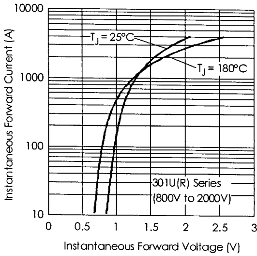
Fig. 13 - Forward Voltage Drop Characteristics
