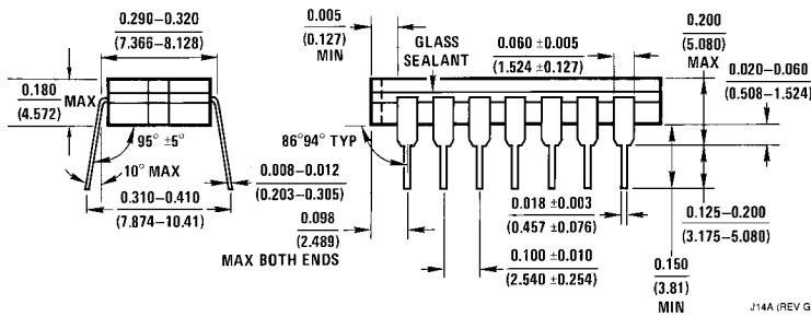
14-Lead Ceramic Dual-In-Line Package (J) Order Number 54LS14DMQB NS Package Number J14A
