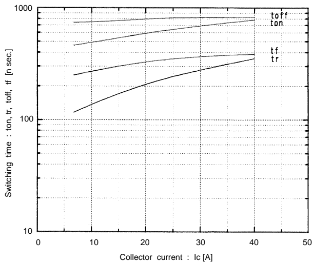
Switching time vs. Collector current V CC =600V, R G =51 ohm, V GE =±15V, T J =25°C
