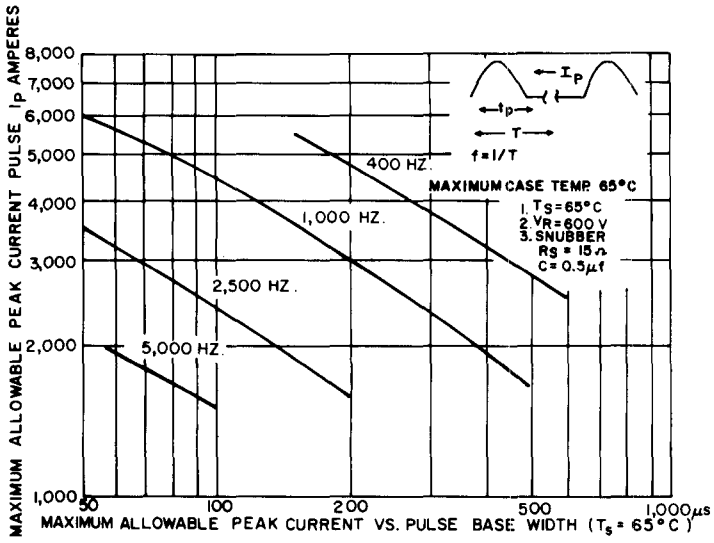
1. MAXIMUM ALLOWABLE PEAK CURRENT VERSUS PULSE BASE WIDTH ( T_s = 65^\circ\text{C} )
