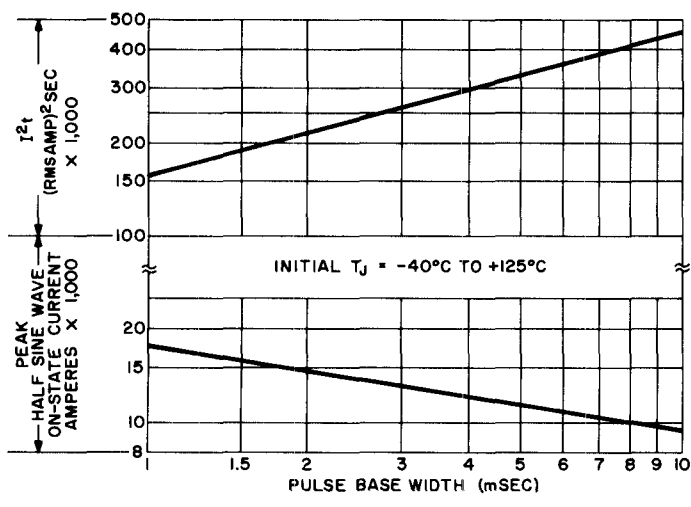
12. SUB-CYCLE SURGE (NON-REPETITIVE) ON-STATE CURRENT AND I 2 t RATING
