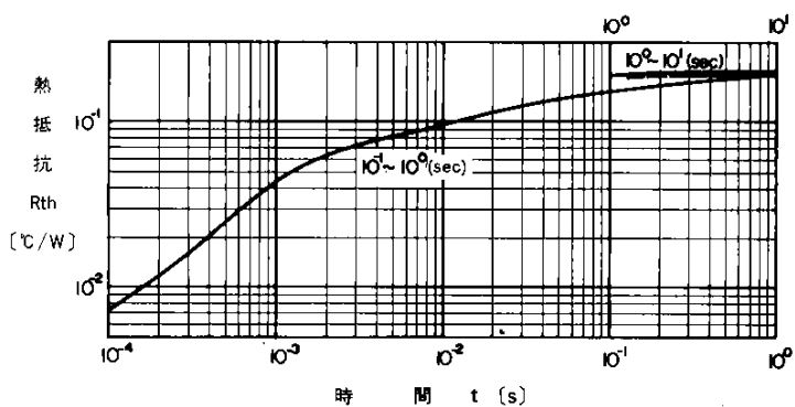
過渡熱抵抗 Transient Thermal Resistance
