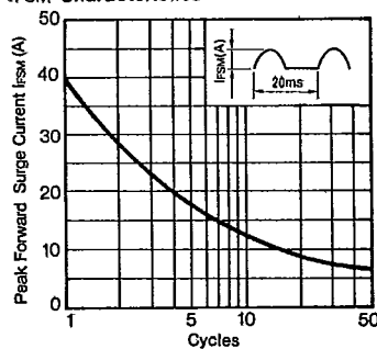
IFSM Characteristics
