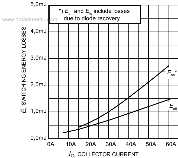
Figure 13. Typical switching energy losses as a function of collector current (inductive load, T_J=150^\circ\text{C} , V_{CE}=400\text{V} , V_{GE}=0/15\text{V} , R_G=11\Omega , Dynamic test circuit in Figure E)
