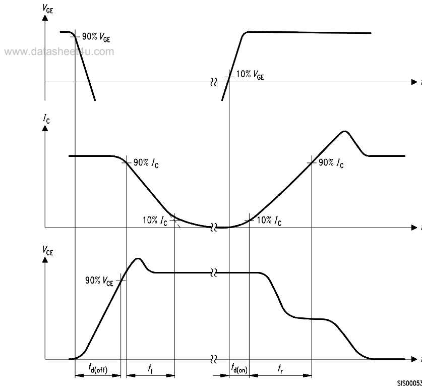
Figure A. Definition of switching times
