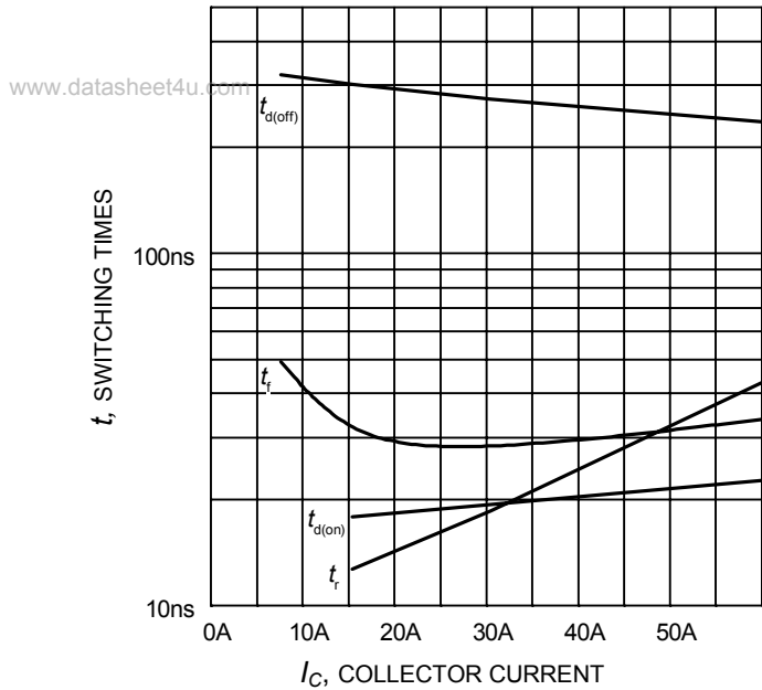
Figure 9. Typical switching times as a function of collector current (inductive load, T_J=150^{\circ}\text{C} , V_{CE}=400\text{V} , V_{GE}=0/15\text{V} , R_G=11\Omega , Dynamic test circuit in Figure E)
