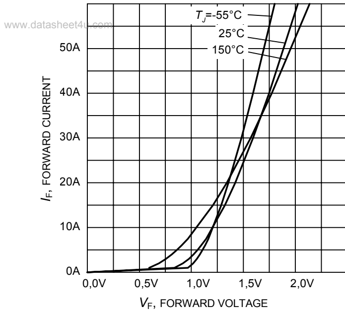
Figure 25. Typical diode forward current as a function of forward voltage
