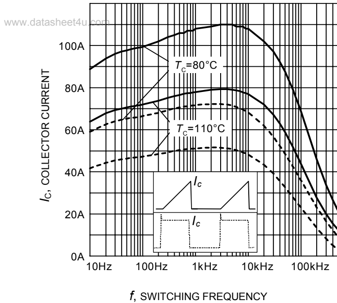
Figure 1. Collector current as a function of switching frequency ( T_j \leq 150^\circ\text{C} , D = 0.5 , V_{CE} = 400\text{V} , V_{GE} = 0/+15\text{V} , R_G = 11\Omega )
