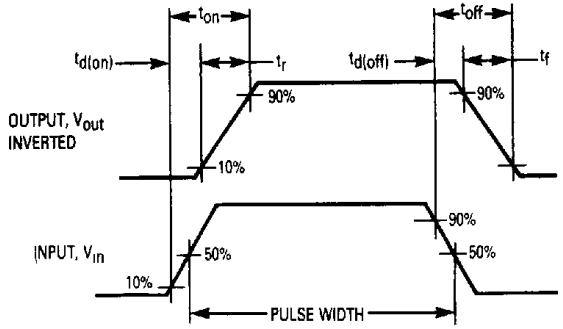
Figure 14. Switching Waveforms
