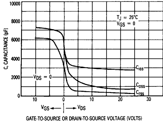
Figure 11. Capacitance Variation
