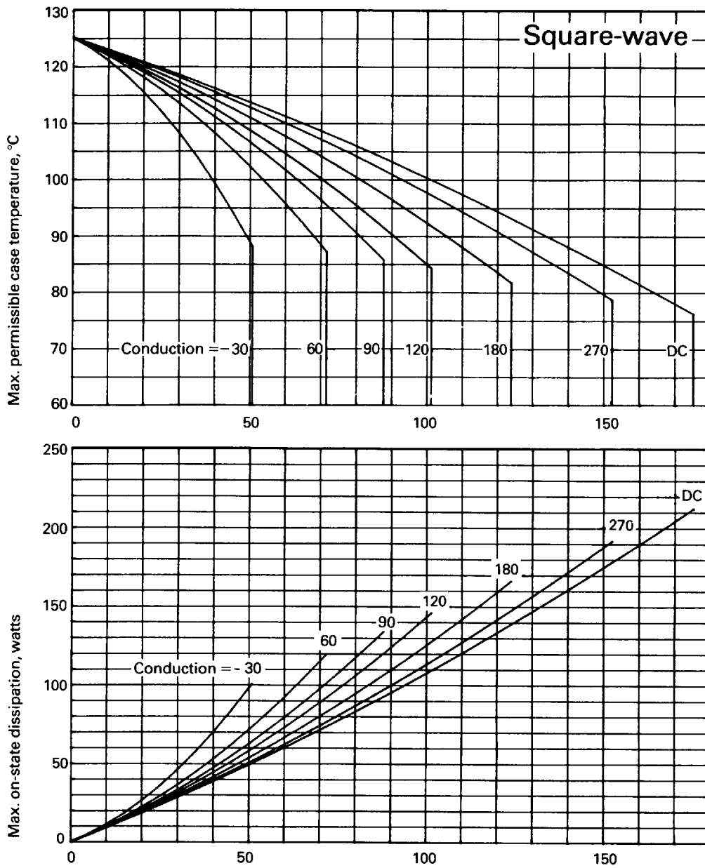
Figure 3 Dissipation and case temperature v. current
