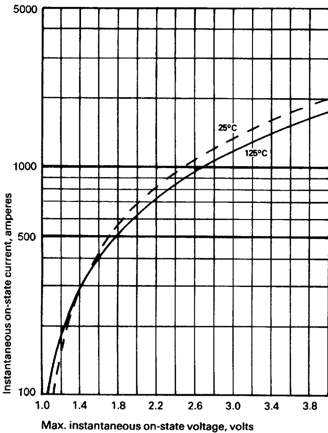
Figure 7 Limit on-state characteristic
