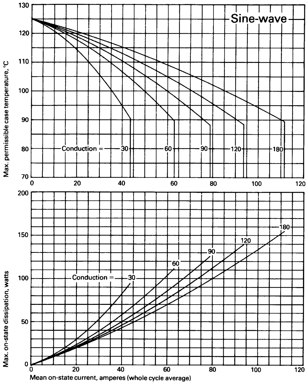
Figure 1 Dissipation and case temperature v. current
