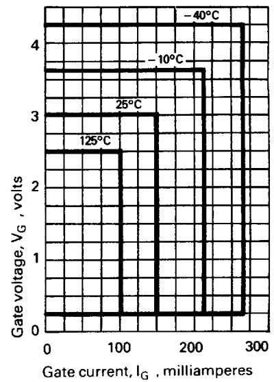
Figure 6 Gate triggering characteristics
