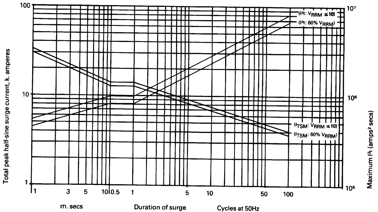
Figure 6 Max. non-repetitive surge current at initial junction temperature 125°C. (gate may temporarily lose control of firing angle) Note: This rating must not be interpreted as an intermittent rating
