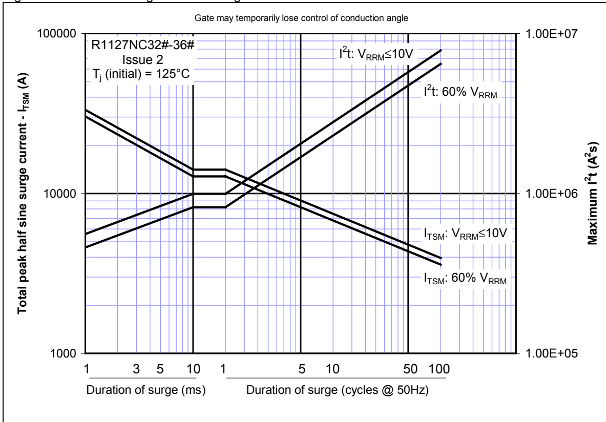
Figure 19 - Maximum surge and I 2 t Ratings
