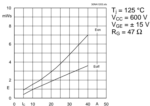
Fig. 3 Turn-on /-off energy = f(I_C)
