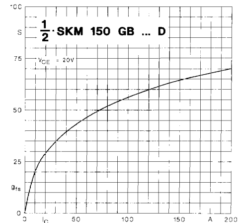
Fig. 31 Forward transconductance
