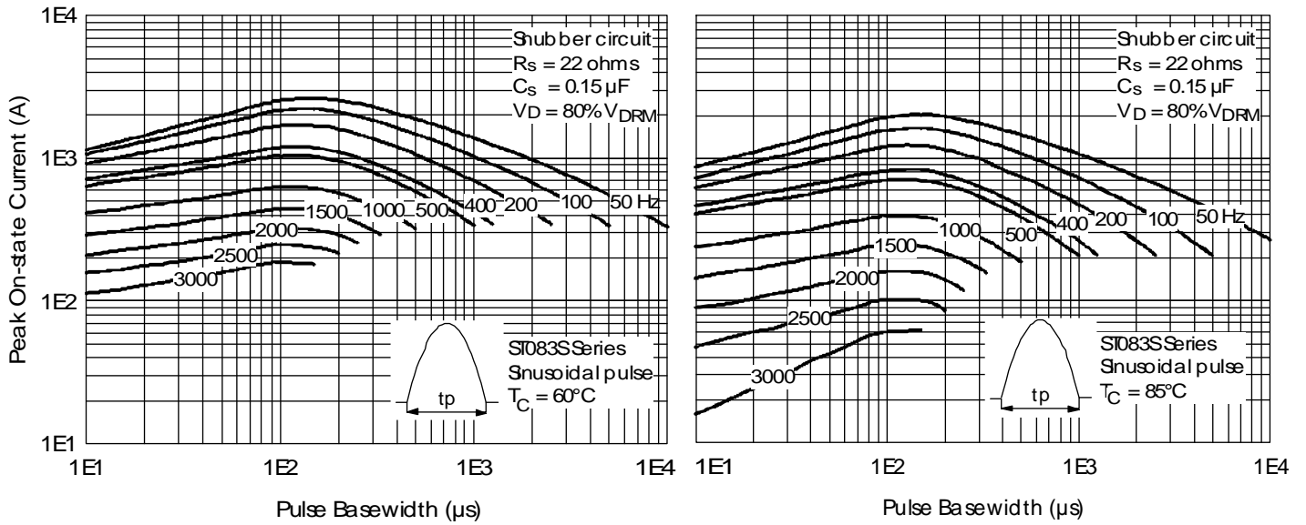
Fig. 11 - Frequency Characteristics
