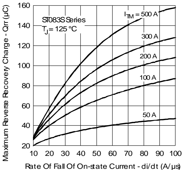
Fig. 9 - Reverse Recovered Charge Characteristics
