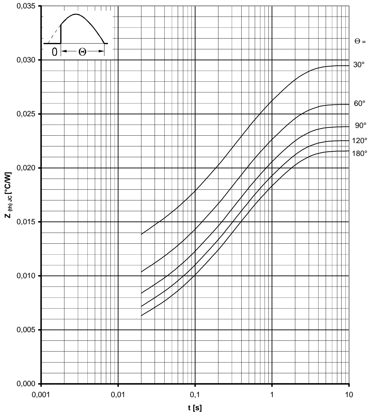
Transienter innerer Wärmewiderstand / Transient thermal impedance Z_{(th)JC} = f(t) Beidseitige Kühlung / Two-sided cooling Parameter: Stromflußwinkel \Theta / current conduction angle \Theta
