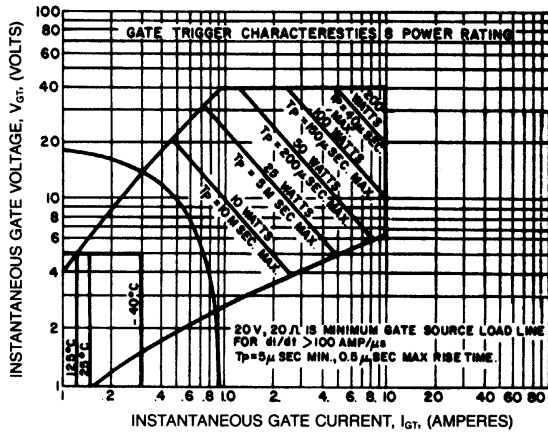
GATE CHARACTERISTICS
